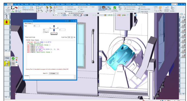
Measurement G-Code cycles are inserted into the CNC program
