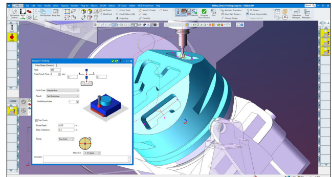
Probing cycles may be defined as GibbsCAM macros
