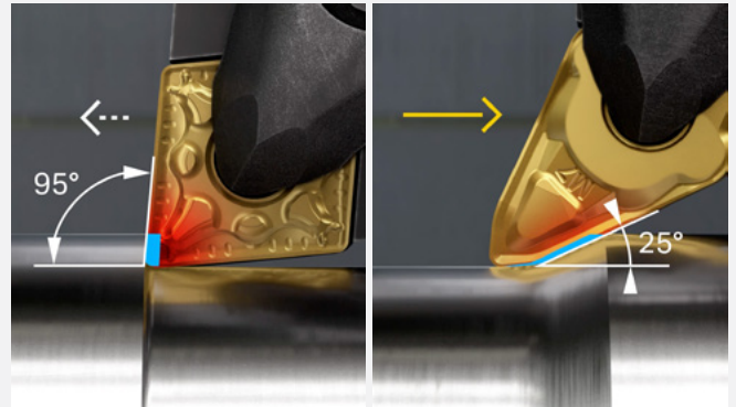
Conventional Turning
